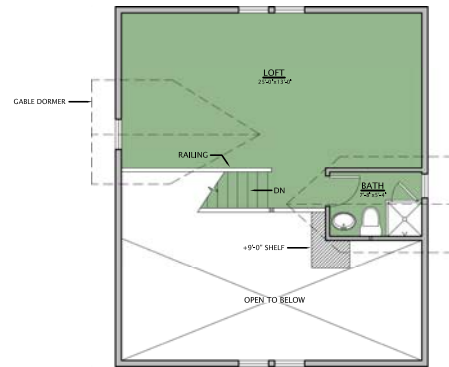
Loft Level Floor Plan
