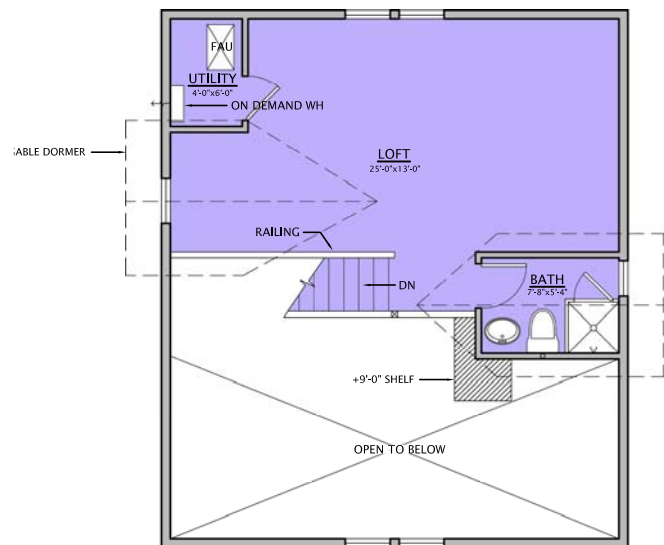
Loft Level Floor Plan
