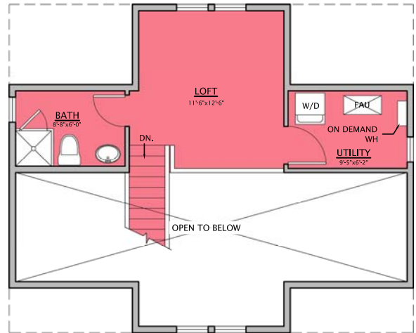
Loft Level Floor Plan
