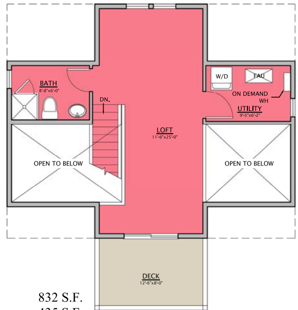
Loft Level Floor Plan
