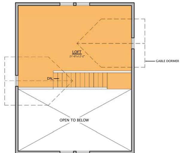
Loft Level Floor Plan
